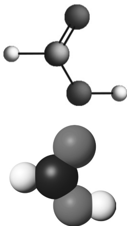
Modele ale moleculei de acid formic
