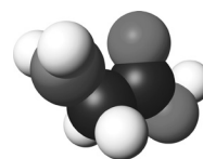
Modelul moleculei de acid aminoacetic
